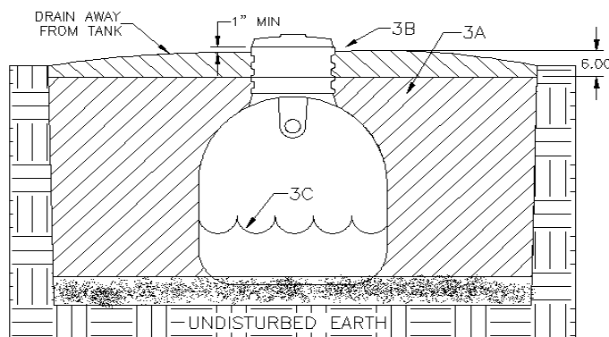
Figure 3: Backfilling
